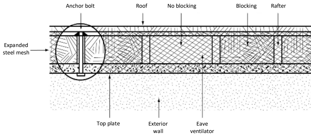
EAVE VENTILATOR
