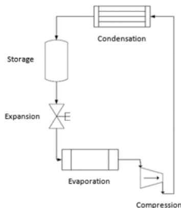
Figure 3: Mechanical Refrigeration Cycle
